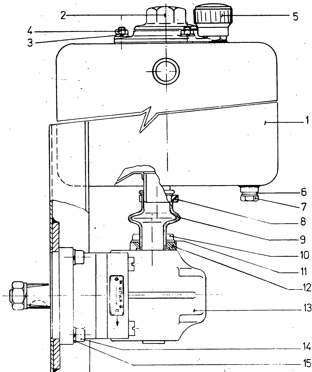
HYDR. POMP, RESERVOIR & FILTER – HYDR' PUMP, RESERVOIR & FILTER POMPE HYDR. RESERVOIR & FILTRE – HYDRAULIKPUMPE, ÖLBEHALTER & FILTER
